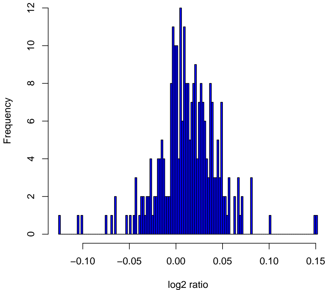
Histogram of log2ratios in 270 HapMap samples at clone Chr10tp-12E1
