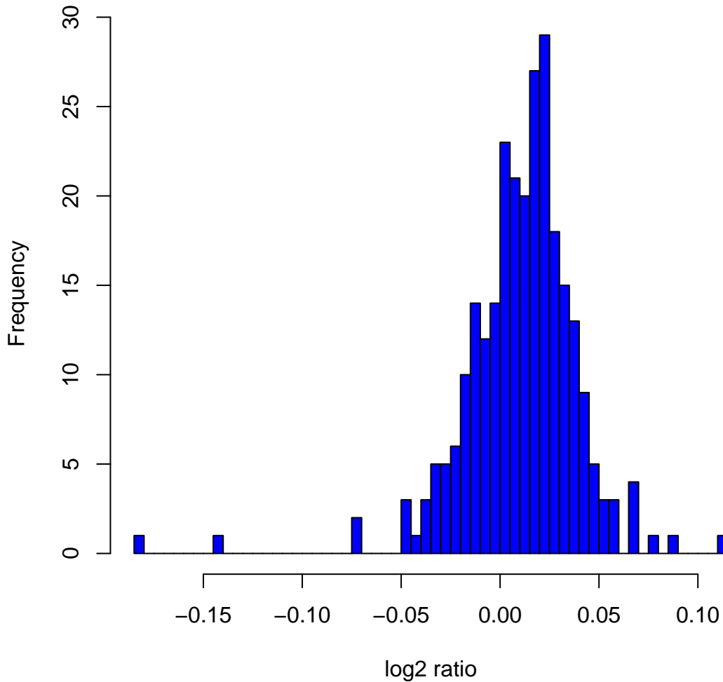
Histogram of log2ratios in 270 HapMap samples at clone Chr10tp-12E3
