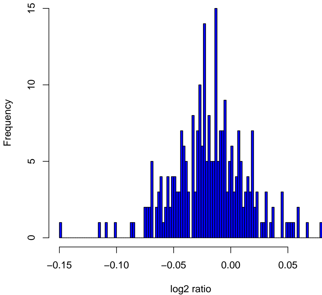
Histogram of log2ratios in 270 HapMap samples at clone Chr10tp-13C11
