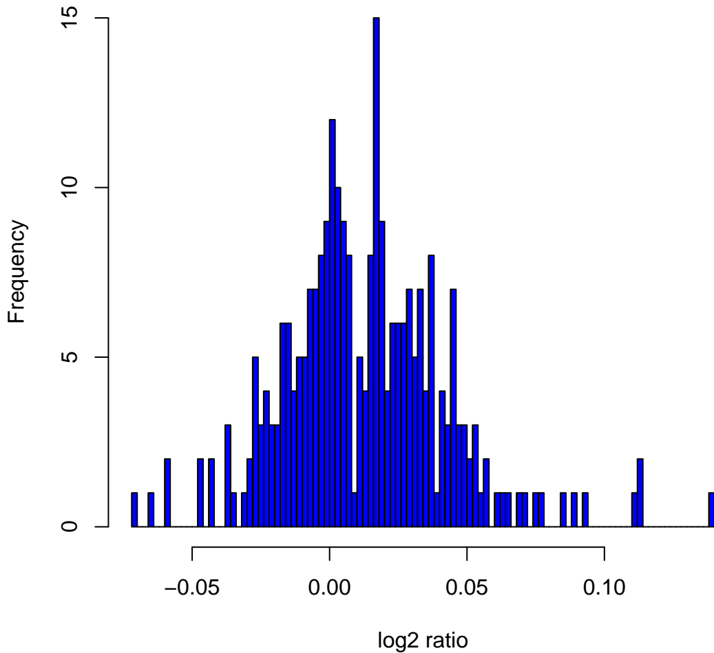
Histogram of log2ratios in 270 HapMap samples at clone Chr10tp-13C9
