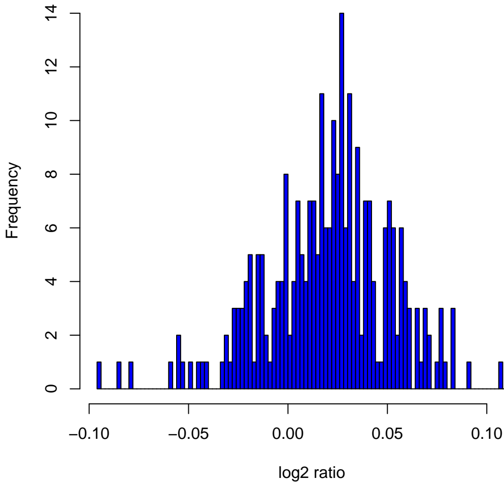
Histogram of log2ratios in 270 HapMap samples at clone Chr10tp-13E2
