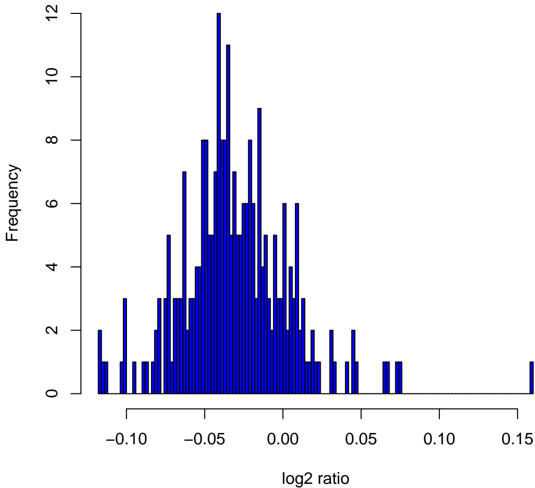
Histogram of \log_2 ratios in 270 HapMap samples at clone Chr10tp-13G12
