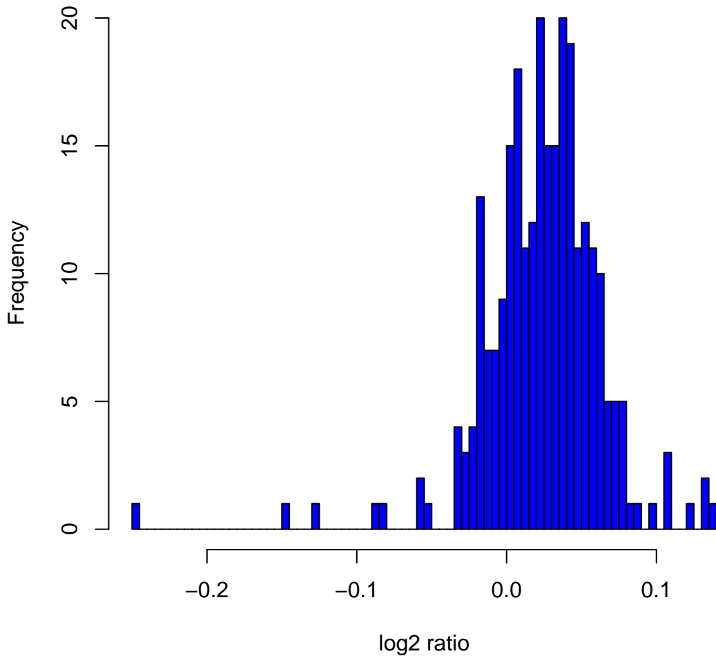
Histogram of log2ratios in 270 HapMap samples at clone Chr10tp-13G2
