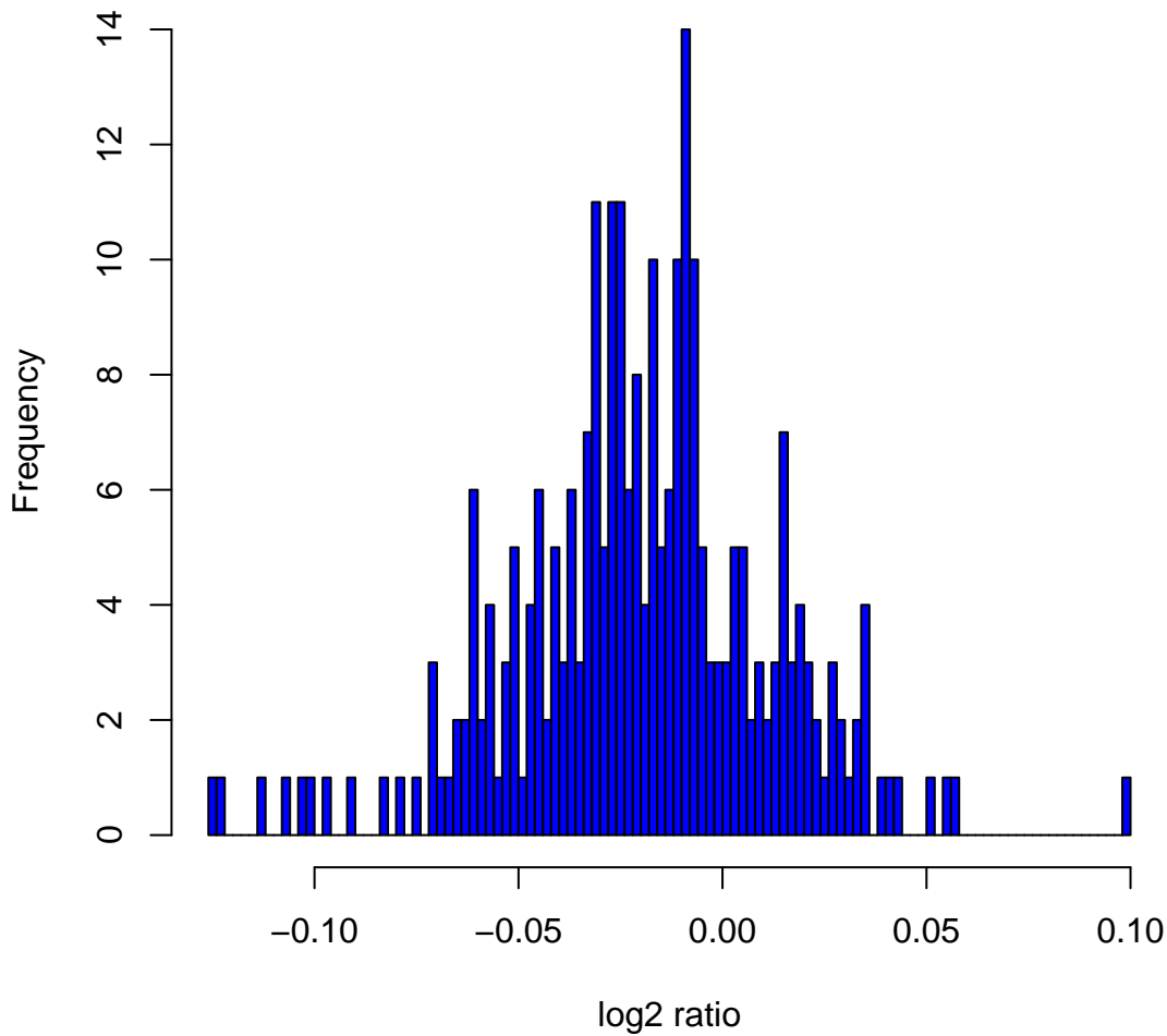
Histogram of log2ratios in 270 HapMap samples at clone Chr10tp-13H10
