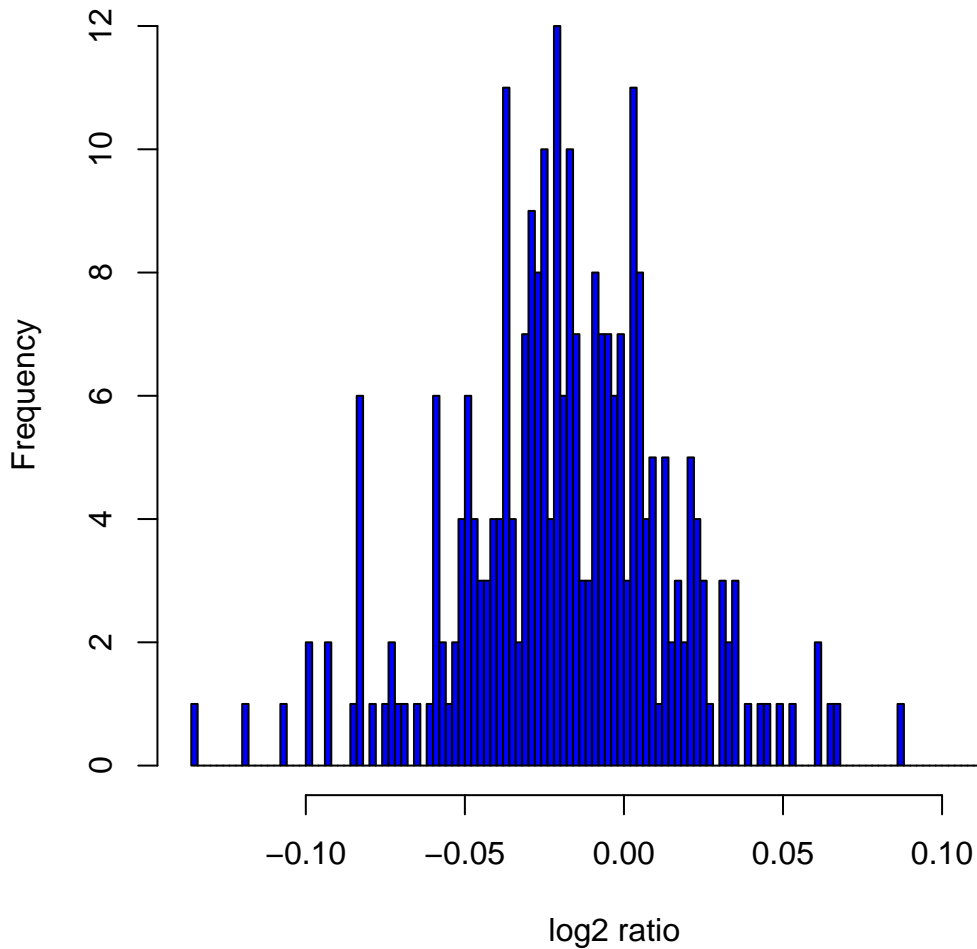
Histogram of log2ratios in 270 HapMap samples at clone Chr10tp-14A8
