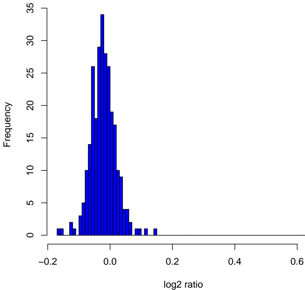
Histogram of log2ratios in 270 HapMap samples at clone Chr10tp-14E6
