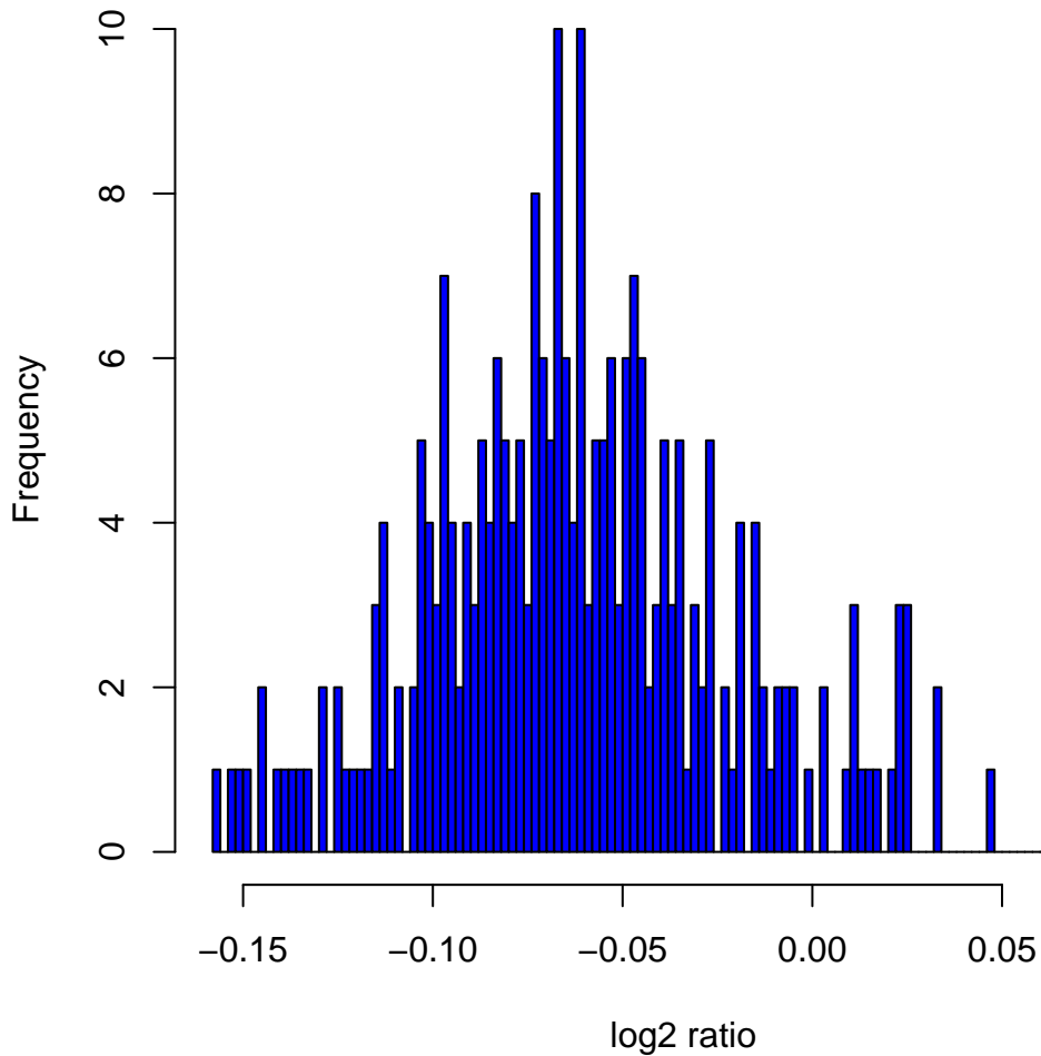
Histogram of log2ratios in 270 HapMap samples at clone Chr10tp-14H5
