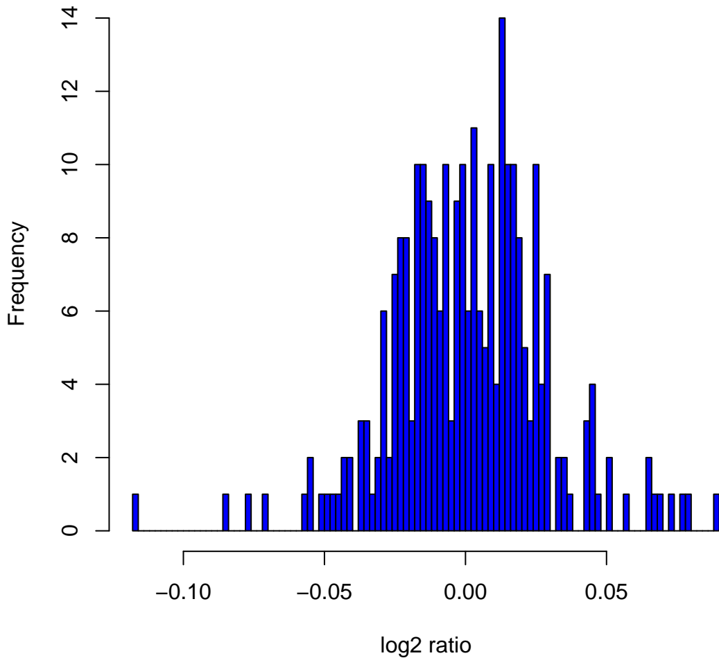
Histogram of log 2 ratios in 270 HapMap samples at clone Chr10tp-15F10
