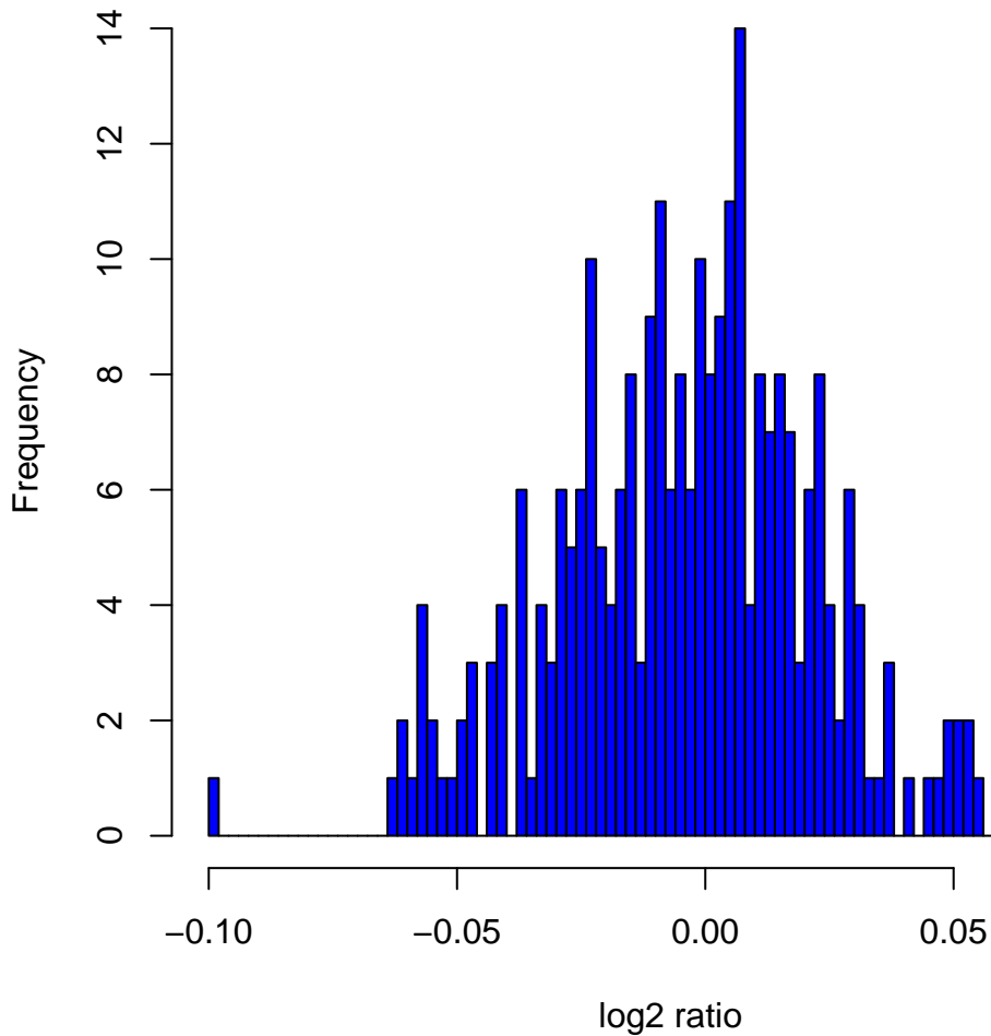
Histogram of log2ratios in 270 HapMap samples at clone Chr10tp-17A3
