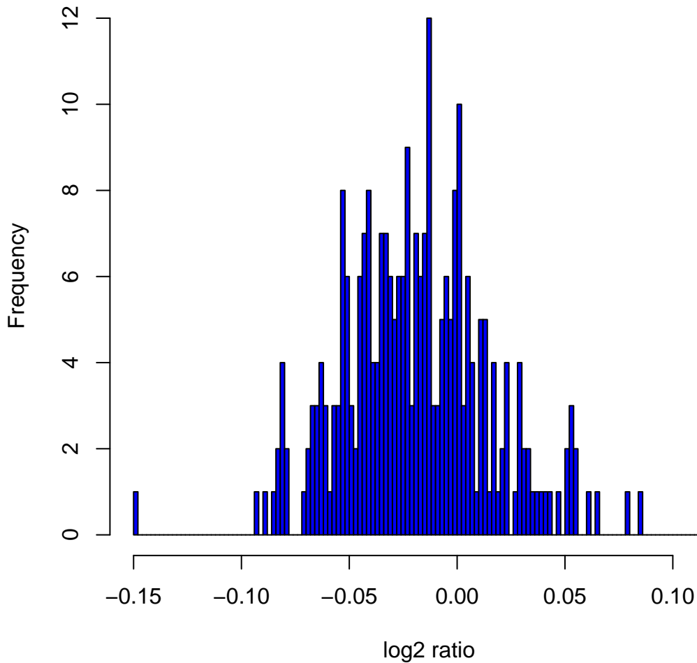
Histogram of log2ratios in 270 HapMap samples at clone Chr10tp-17C2
