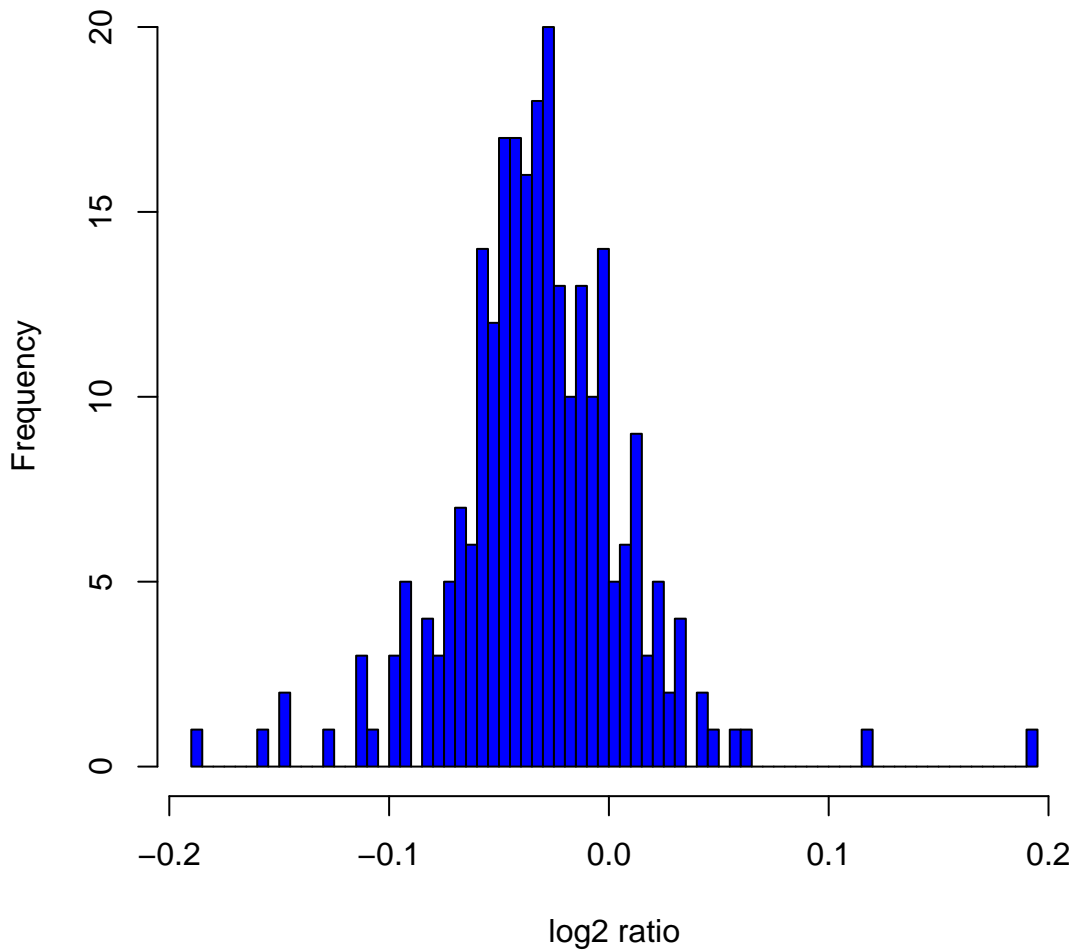
Histogram of log2ratios in 270 HapMap samples at clone Chr10tp-18A10
