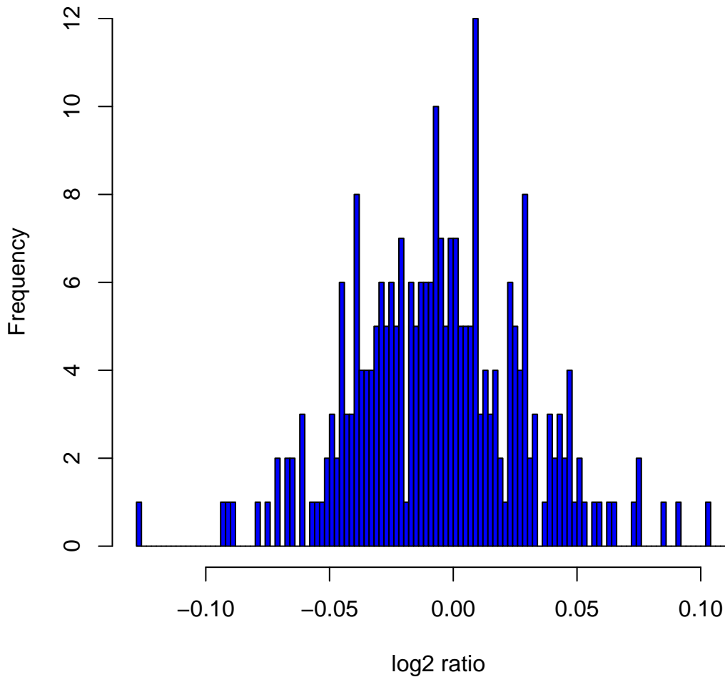
Histogram of log 2 ratios in 270 HapMap samples at clone Chr10tp-1B8
