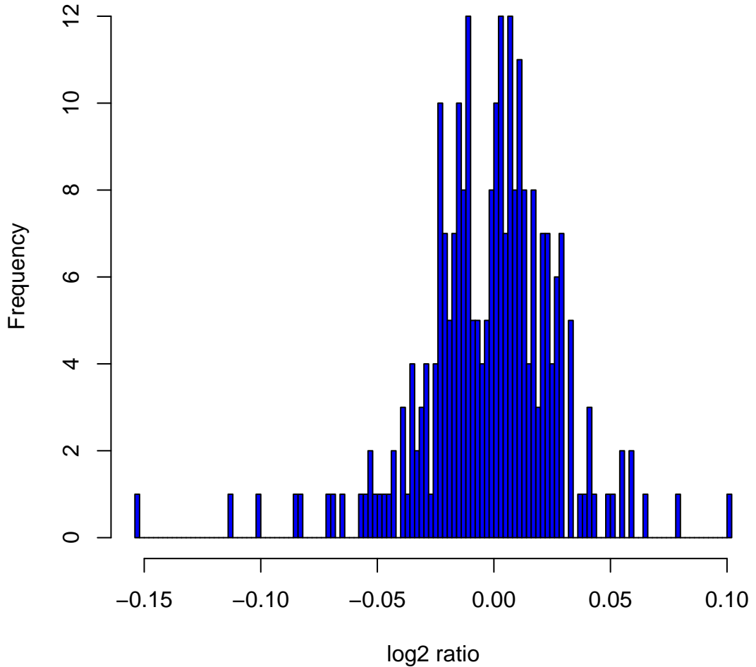
Histogram of log2ratios in 270 HapMap samples at clone Chr10tp-1C11
