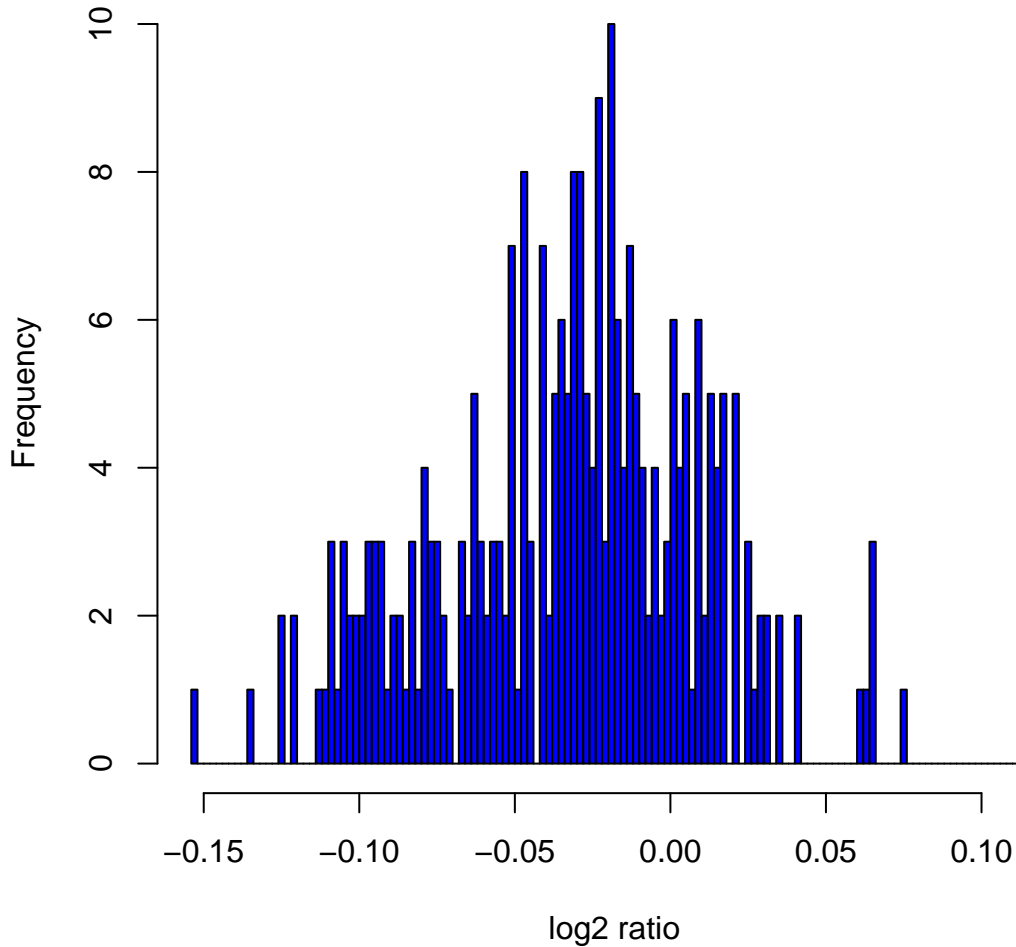
Histogram of log2ratios in 270 HapMap samples at clone Chr10tp-1D12
