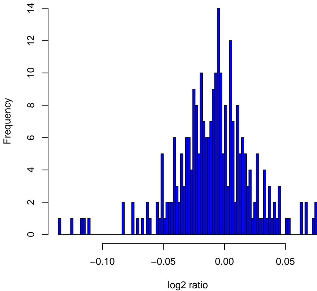
Histogram of log 2 ratios in 270 HapMap samples at clone Chr10tp-1D3
