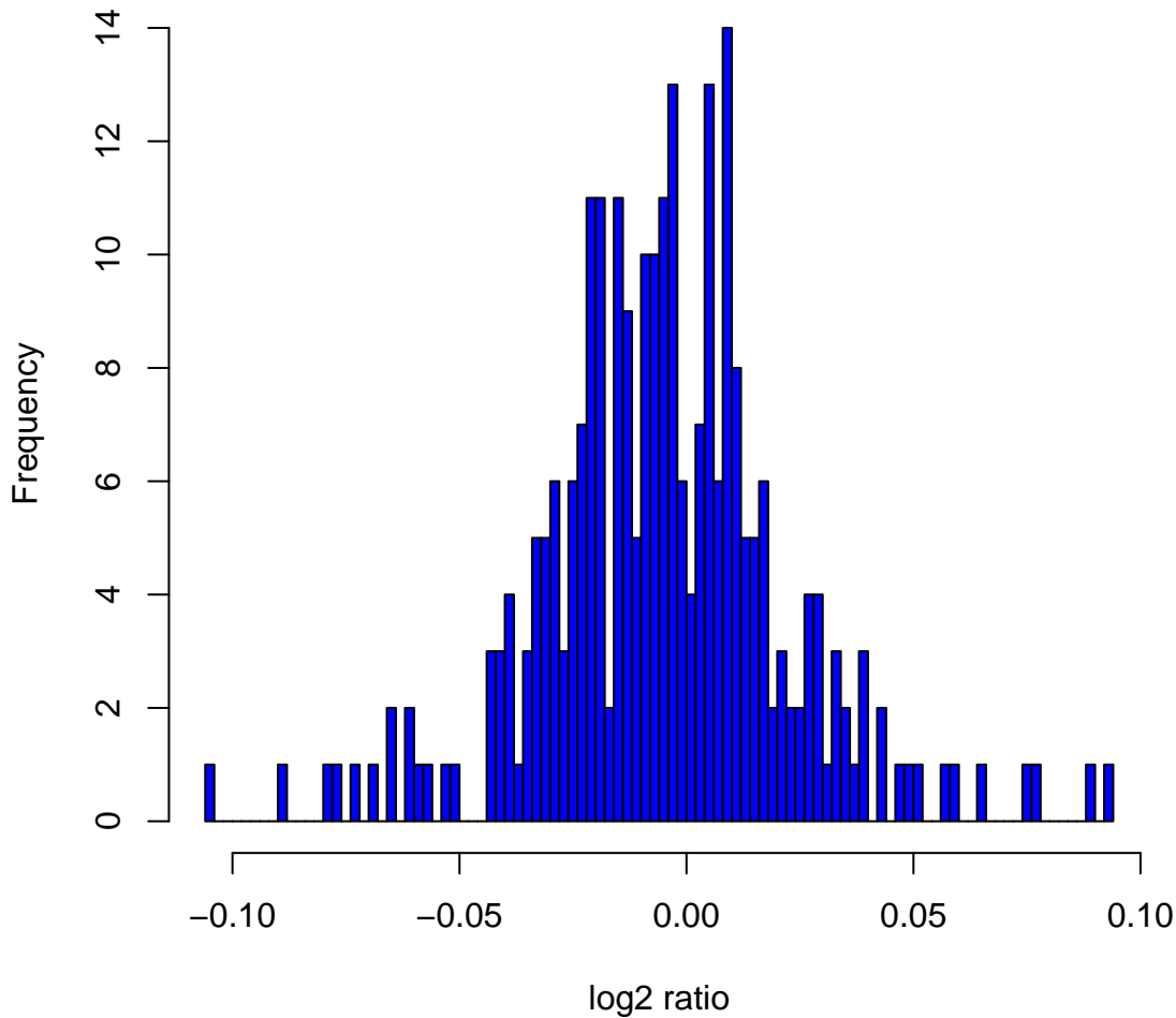
Histogram of log 2 ratios in 270 HapMap samples at clone Chr10tp-1E5
