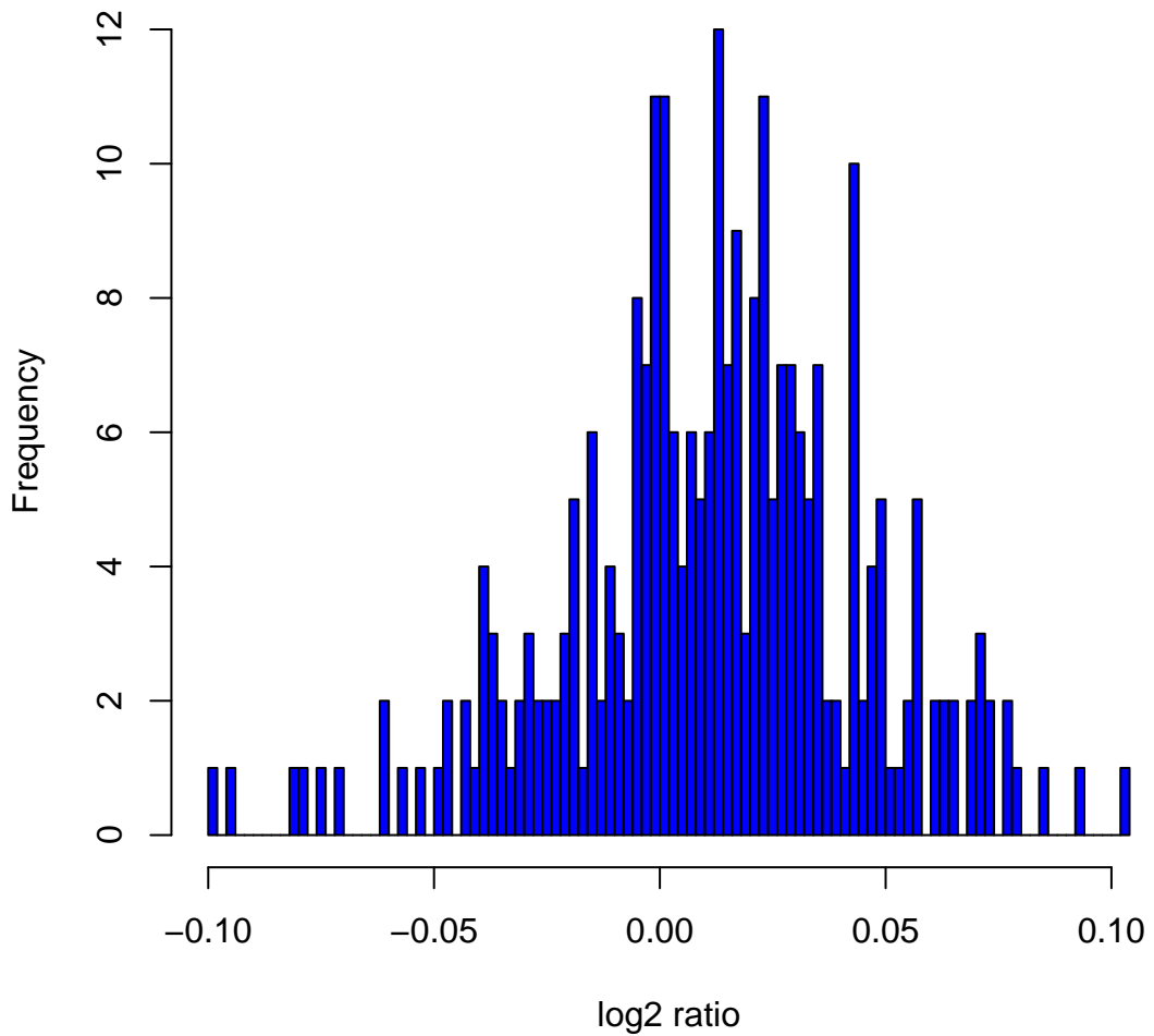
Histogram of log 2 ratios in 270 HapMap samples at clone Chr10tp-1E6
