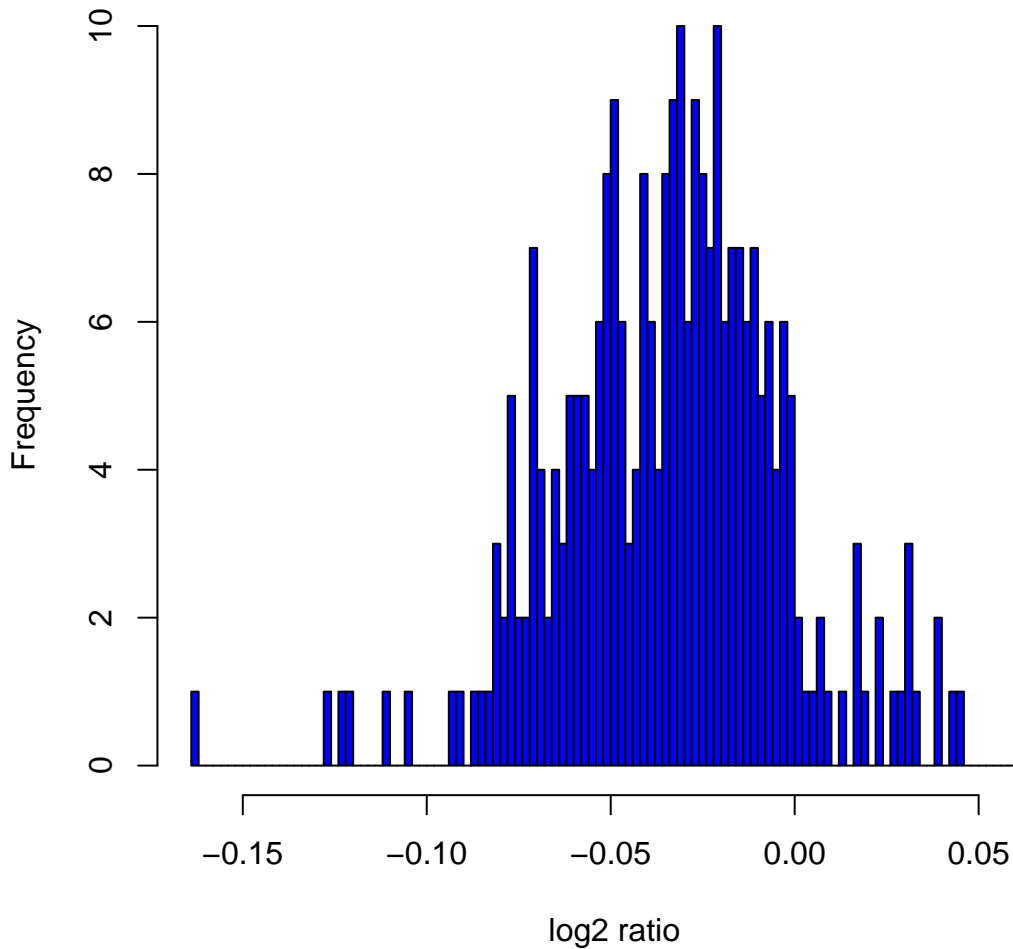
Histogram of log 2 ratios in 270 HapMap samples at clone Chr10tp-1G1
