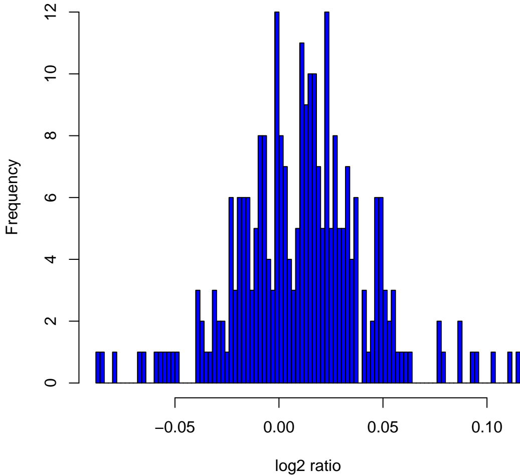
Histogram of log2ratios in 270 HapMap samples at clone Chr10tp-1G2
