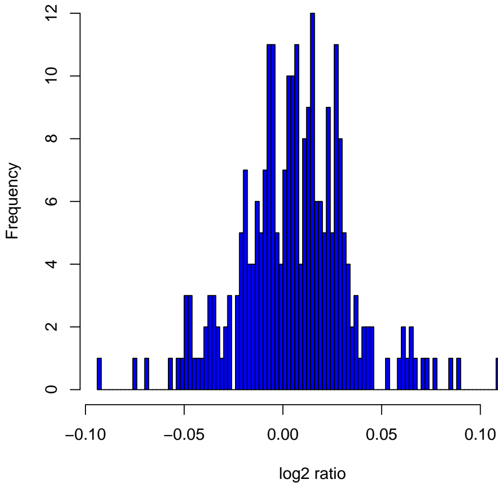
Histogram of log2ratios in 270 HapMap samples at clone Chr10tp-1H12
