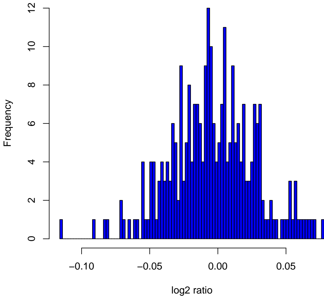
Histogram of log2ratios in 270 HapMap samples at clone Chr10tp-2D9
