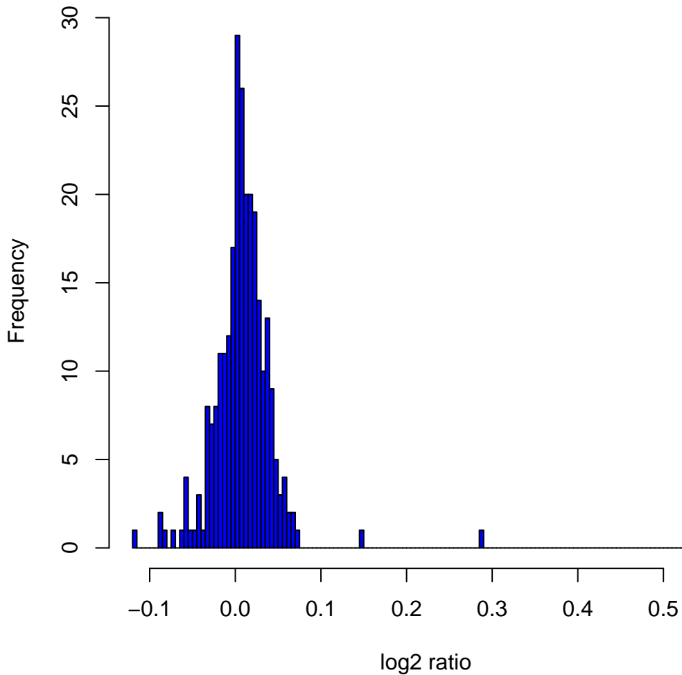
Histogram of log2ratios in 270 HapMap samples at clone Chr10tp-2E12
