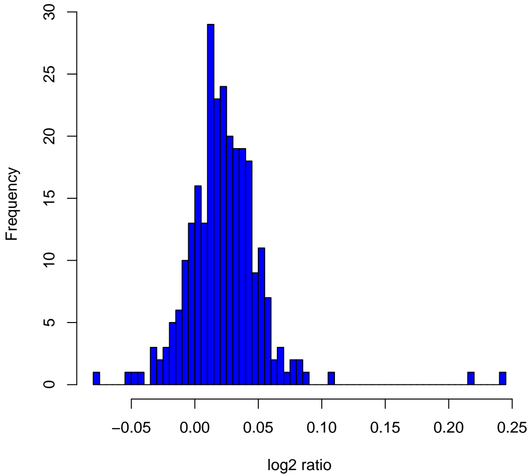
Histogram of log2ratios in 270 HapMap samples at clone Chr10tp-2H1
