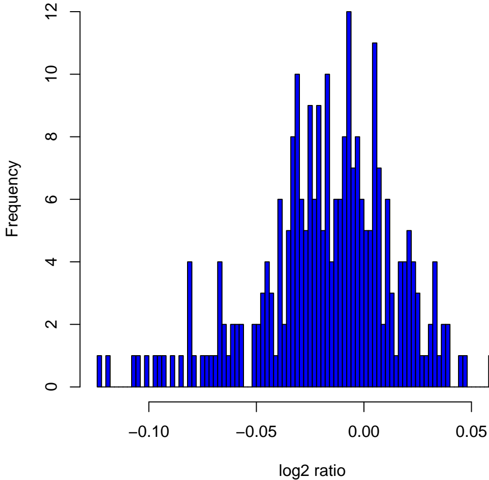
Histogram of log2ratios in 270 HapMap samples at clone Chr10tp-3D11
