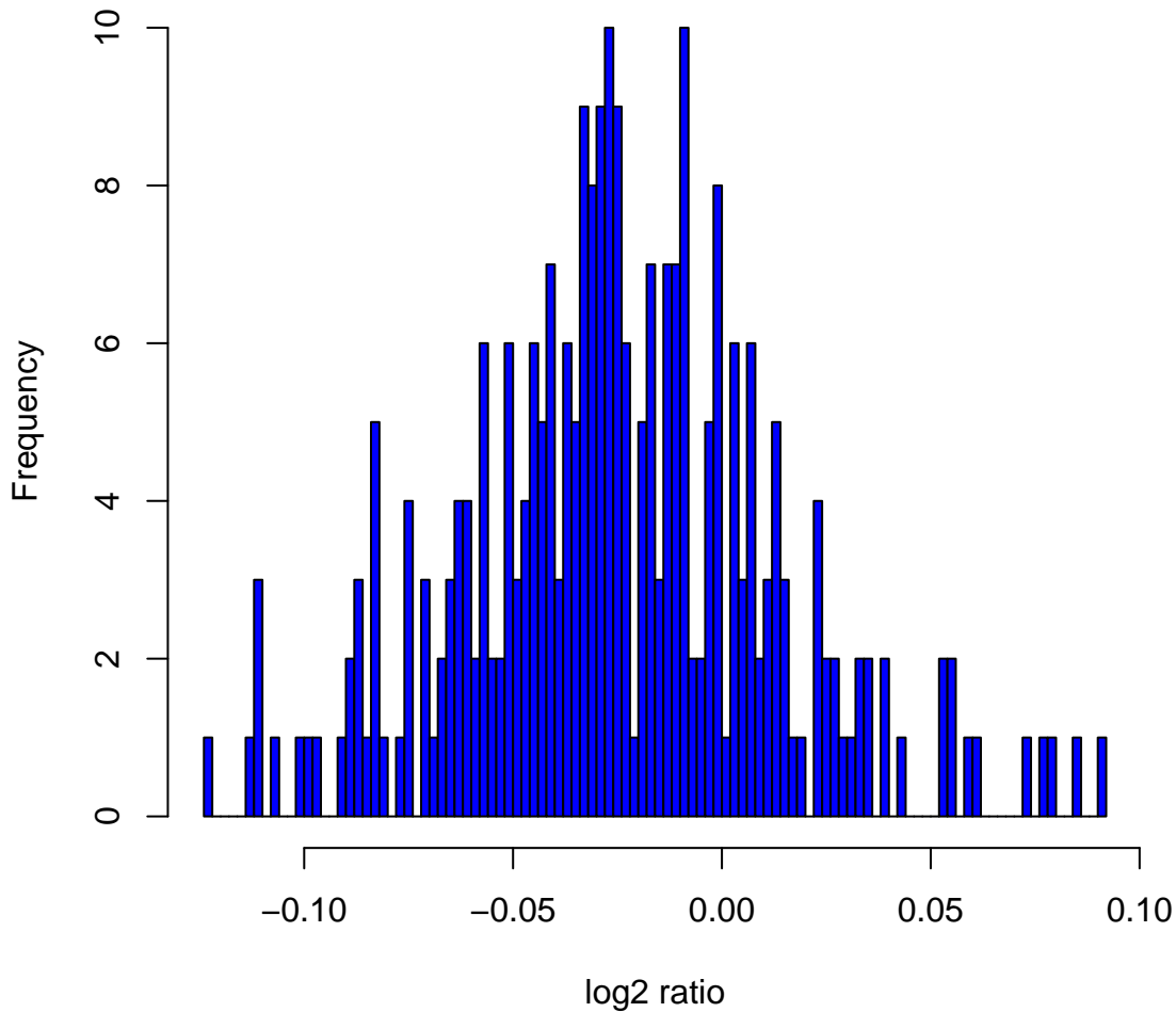
Histogram of \log_2 ratios in 270 HapMap samples at clone Chr10tp-3G12
