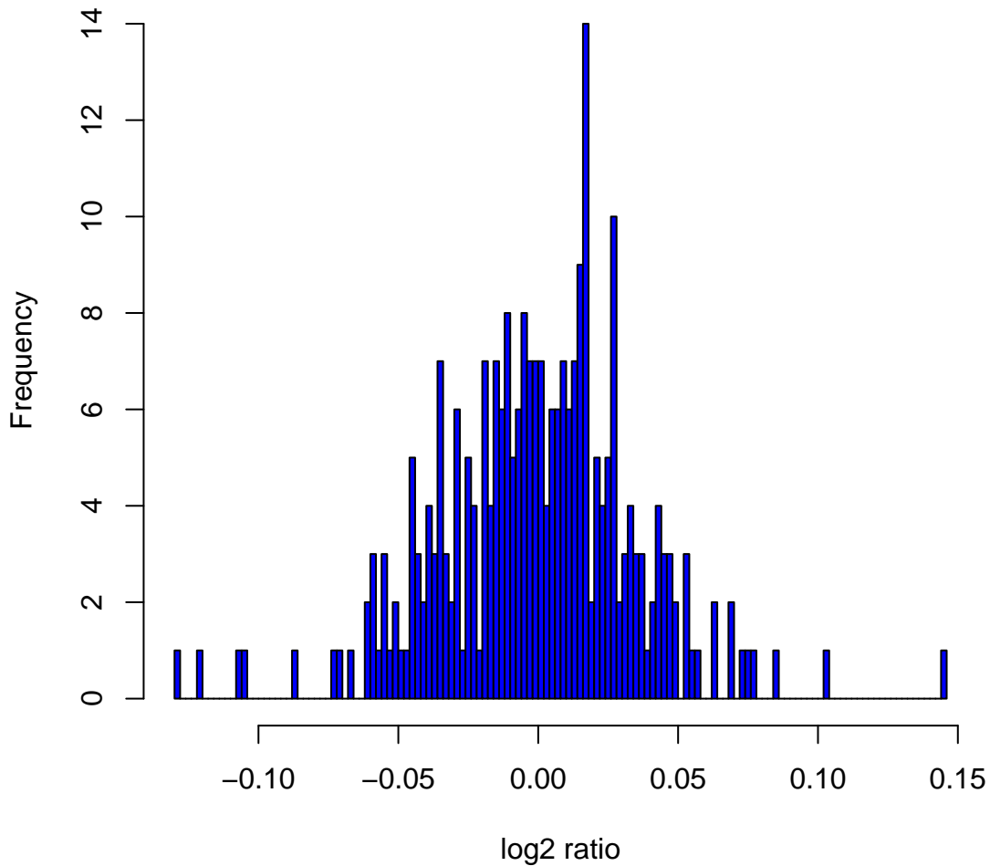
Histogram of \log_2 ratios in 270 HapMap samples at clone Chr10tp-3G5
