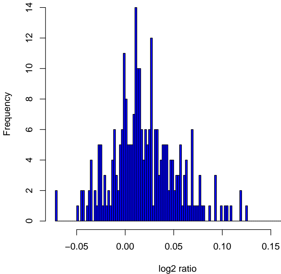
Histogram of log2ratios in 270 HapMap samples at clone Chr10tp-3H10
