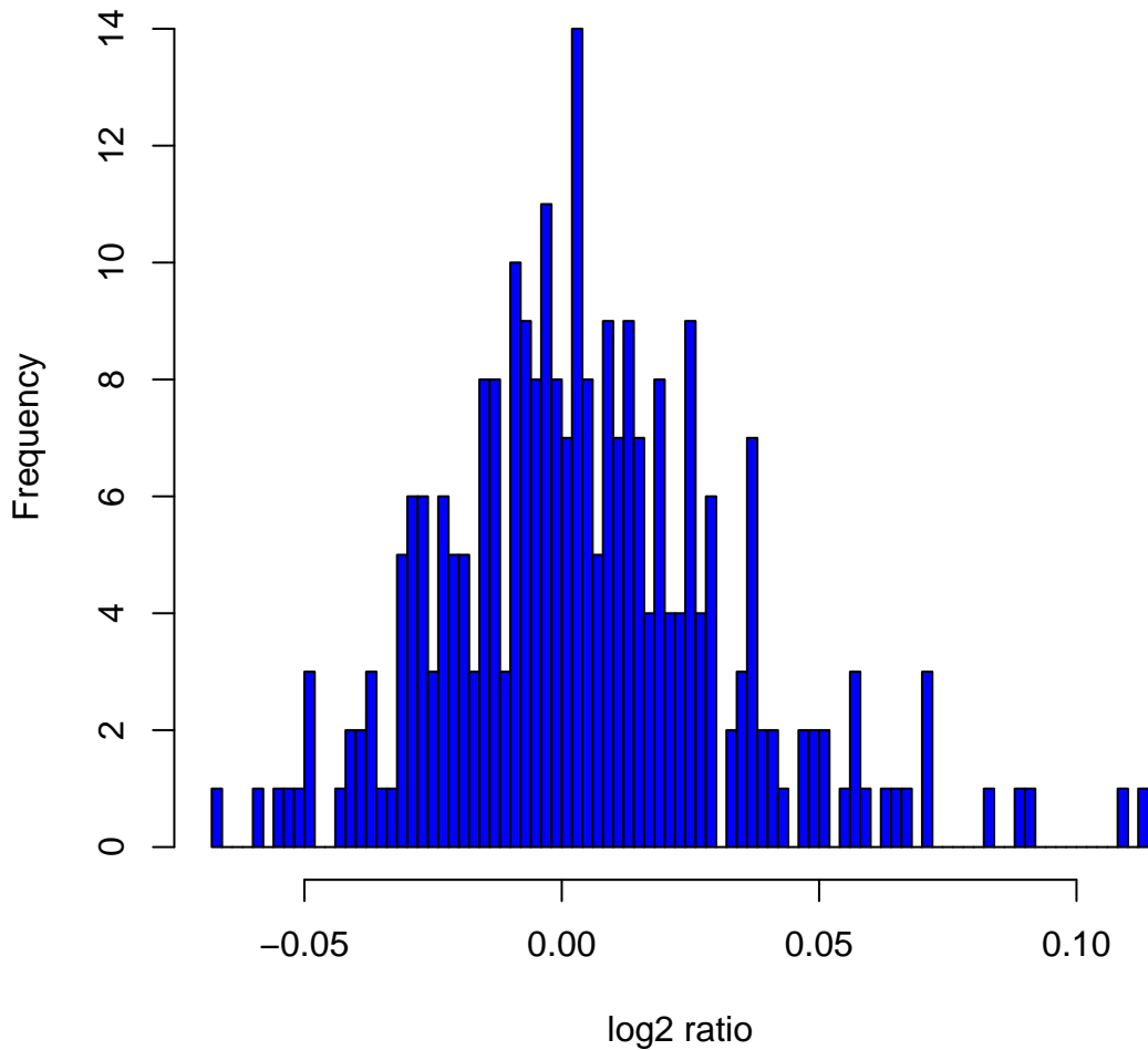
Histogram of log 2 ratios in 270 HapMap samples at clone Chr10tp-4D3
