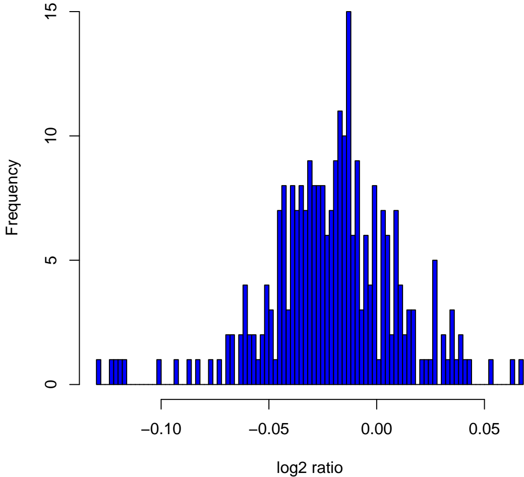
Histogram of log2ratios in 270 HapMap samples at clone Chr10tp-4G7
