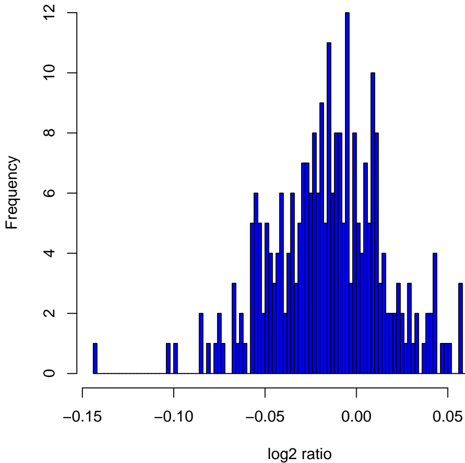
Histogram of log 2 ratios in 270 HapMap samples at clone Chr10tp-4G9
