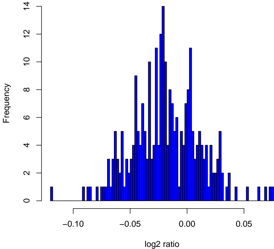
Histogram of log2ratios in 270 HapMap samples at clone Chr10tp-4H11
