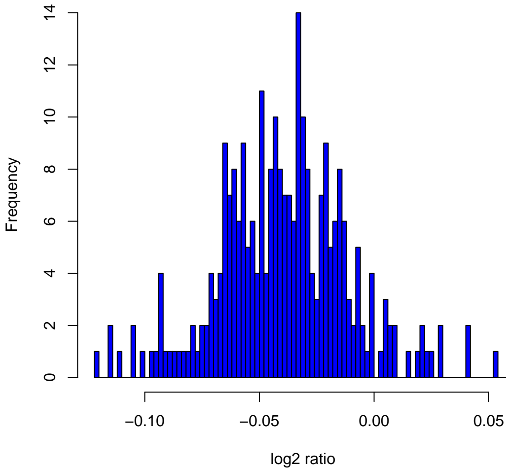
Histogram of log 2 ratios in 270 HapMap samples at clone Chr10tp-5A2
