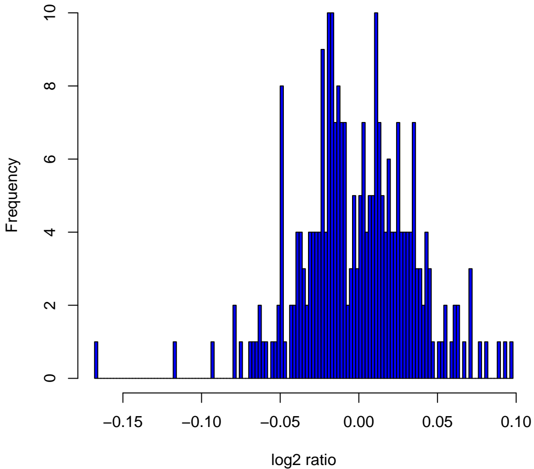
Histogram of log2ratios in 270 HapMap samples at clone Chr10tp-5B10
