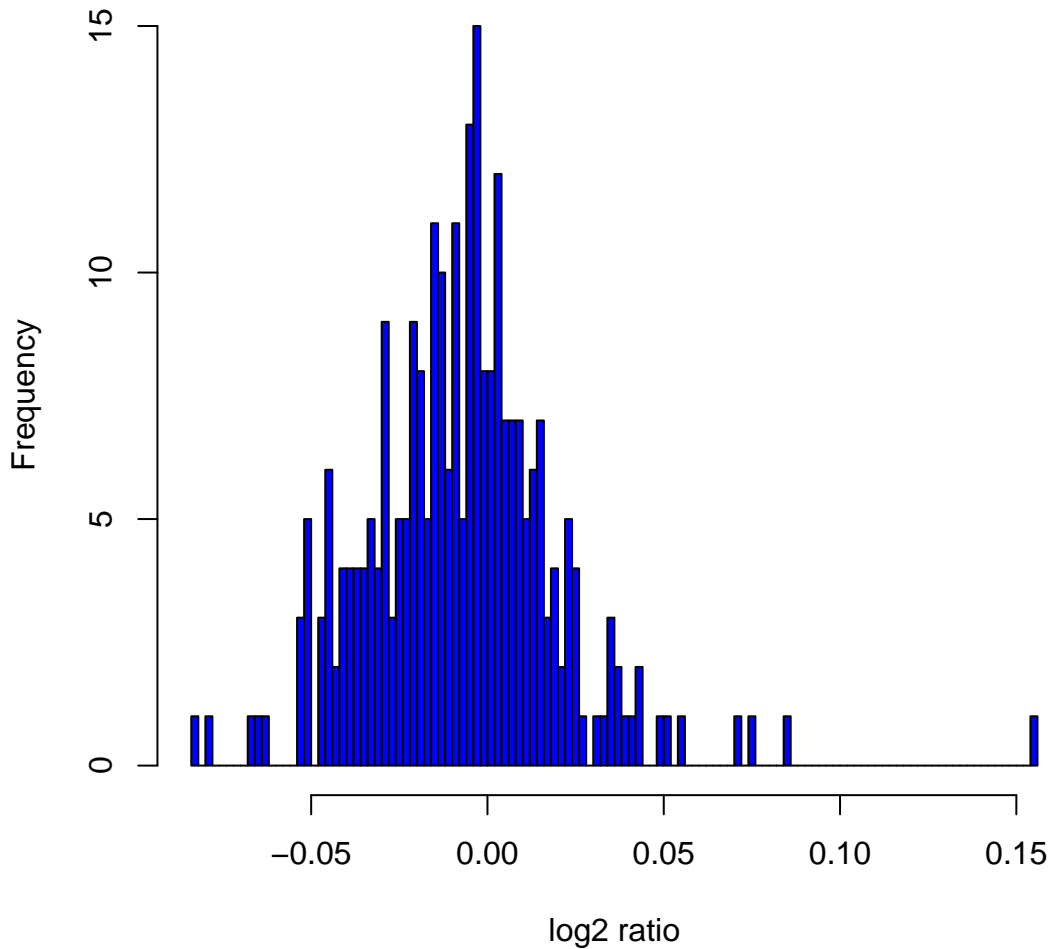
Histogram of log2ratios in 270 HapMap samples at clone Chr10tp-5E11
