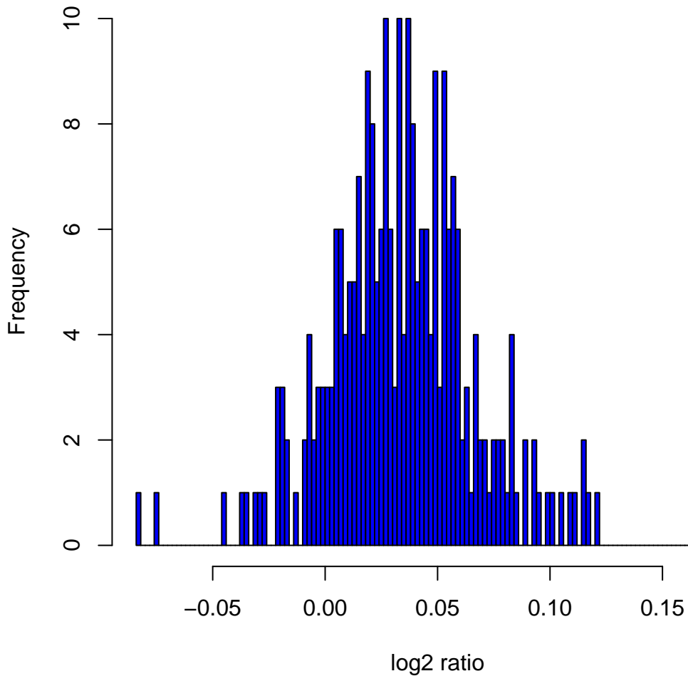
Histogram of log2ratios in 270 HapMap samples at clone Chr10tp-5G5
