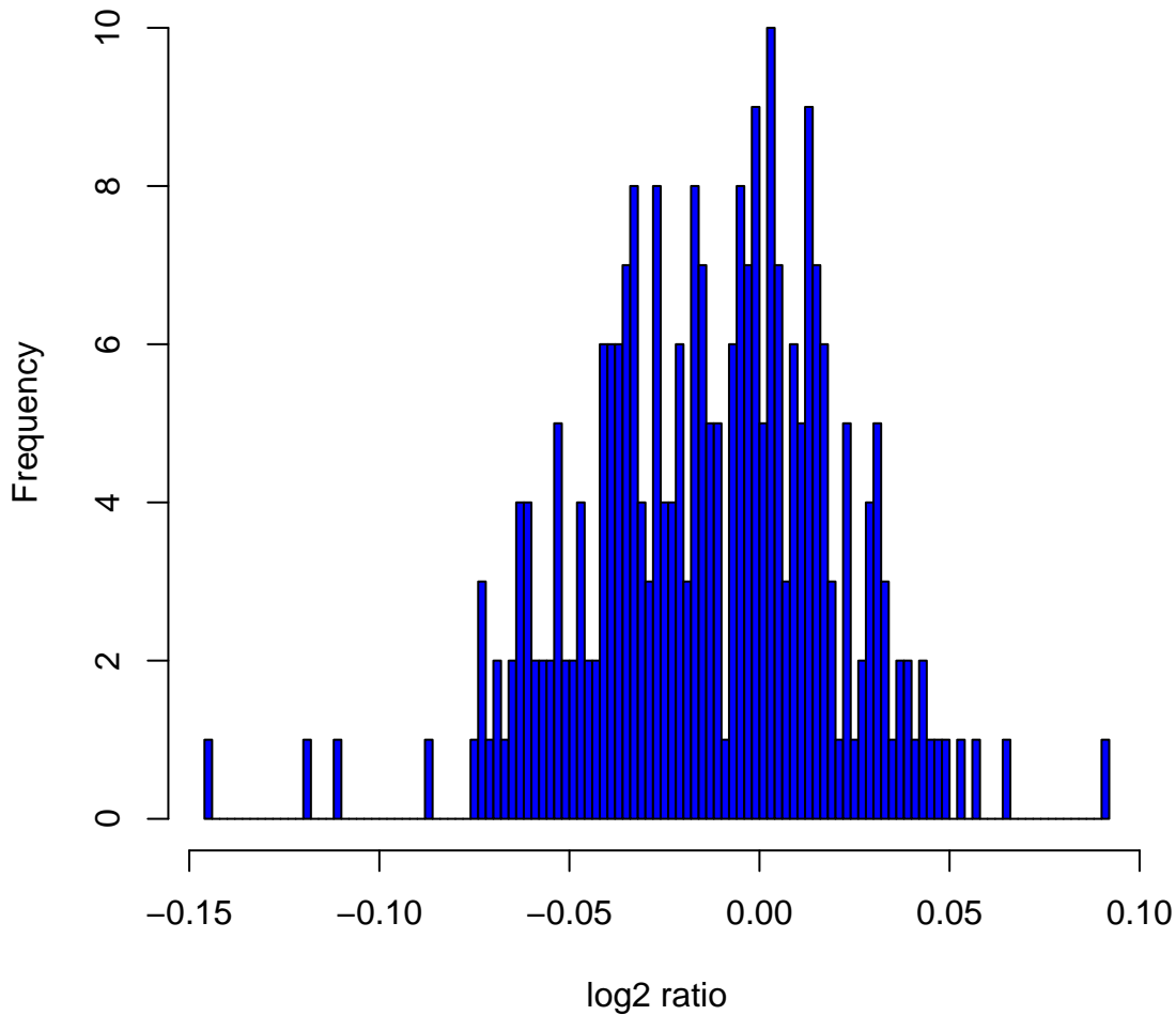
Histogram of log 2 ratios in 270 HapMap samples at clone Chr10tp-5H4
