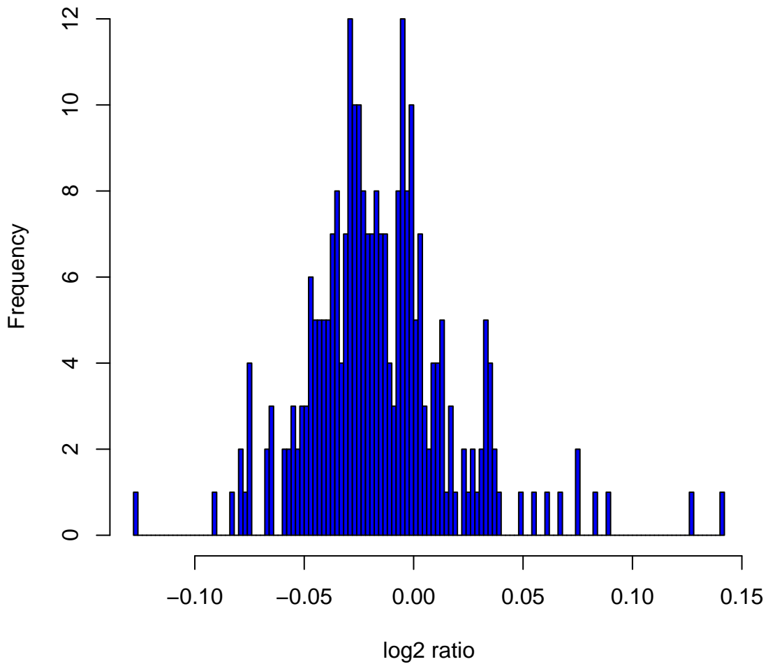
Histogram of log 2 ratios in 270 HapMap samples at clone Chr10tp-6E5
