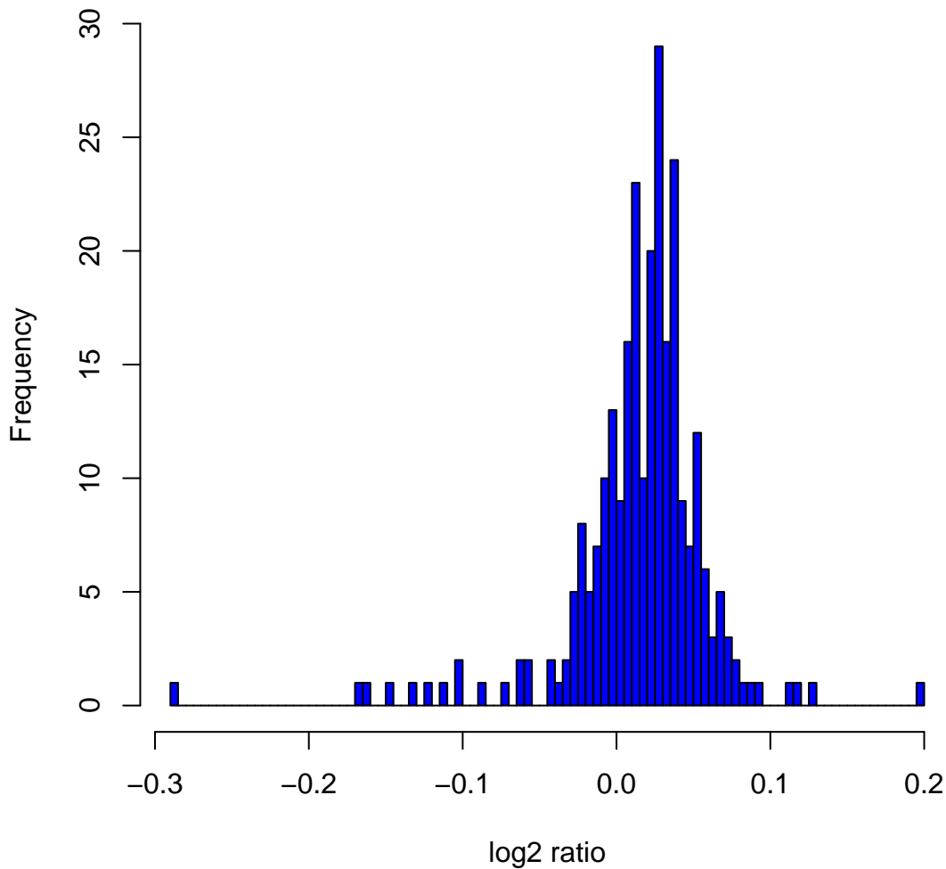
Histogram of log2ratios in 270 HapMap samples at clone Chr10tp-6G1
