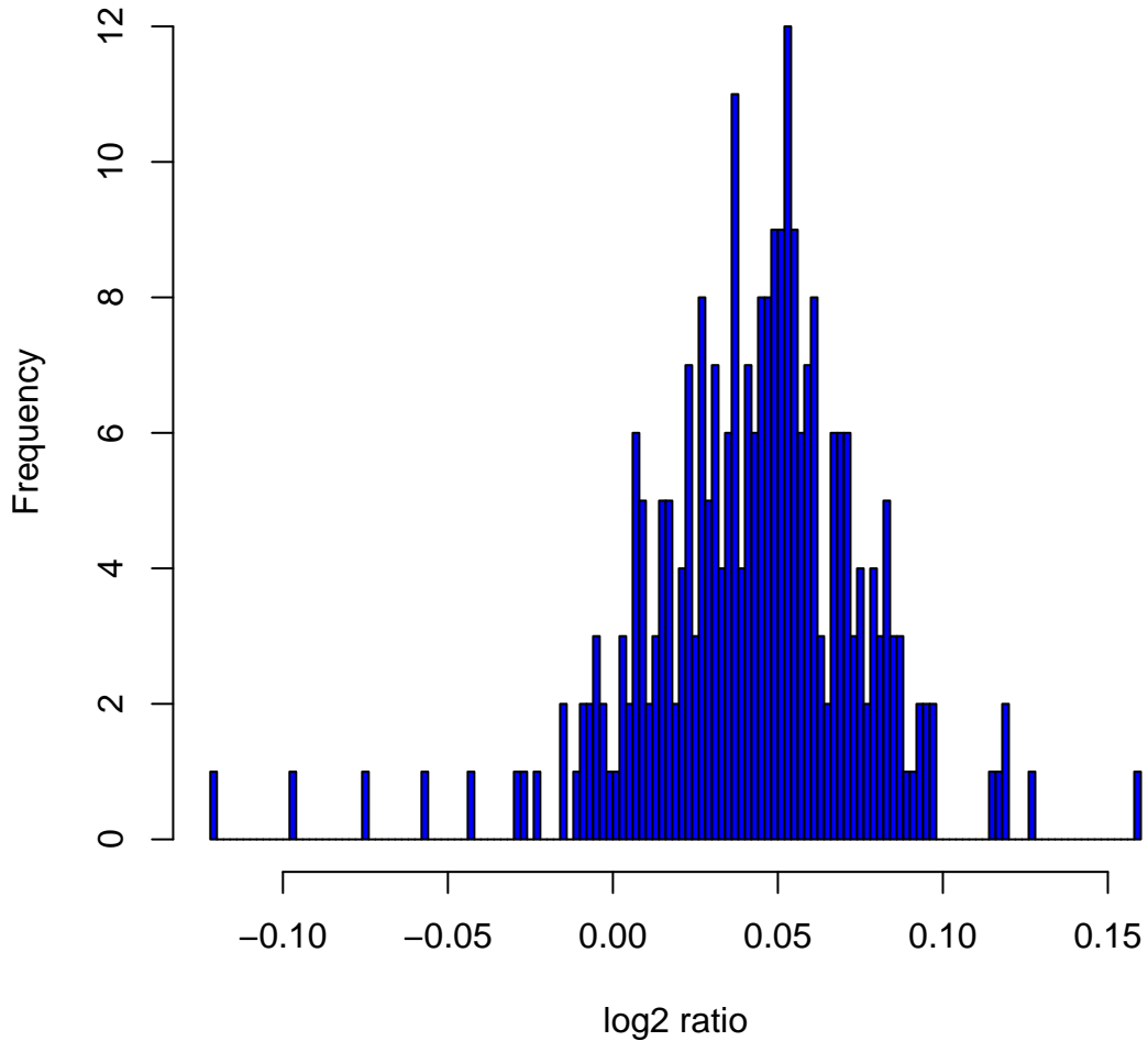
Histogram of log 2 ratios in 270 HapMap samples at clone Chr10tp-6G7
