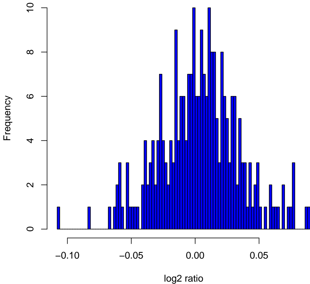
Histogram of log2ratios in 270 HapMap samples at clone Chr10tp-7D11
