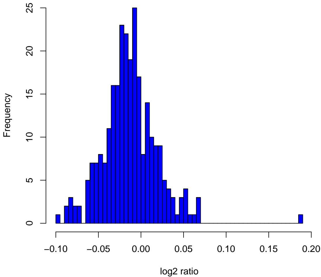
Histogram of log 2 ratios in 270 HapMap samples at clone Chr10tp-7E5
