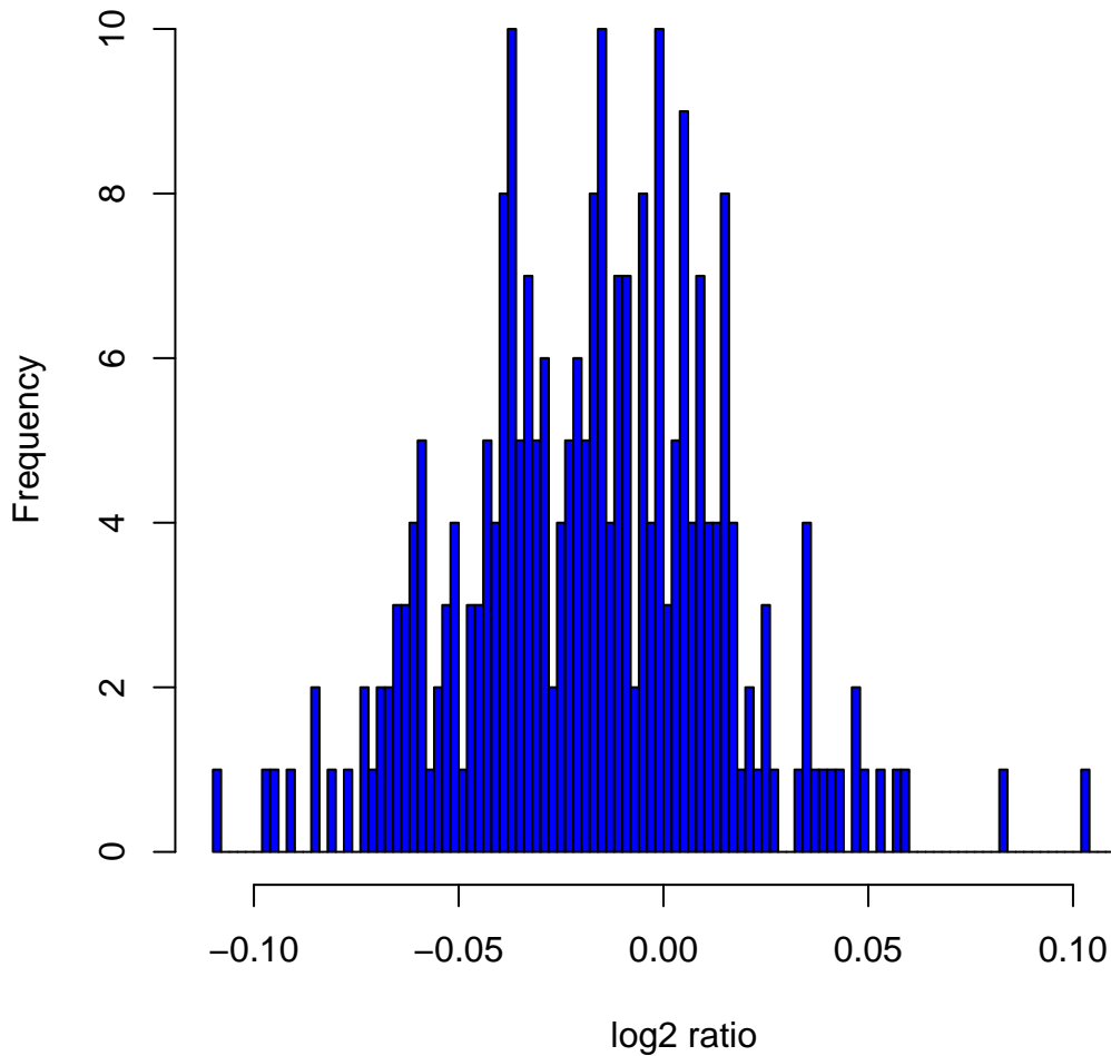
Histogram of log 2 ratios in 270 HapMap samples at clone Chr10tp-7F6
