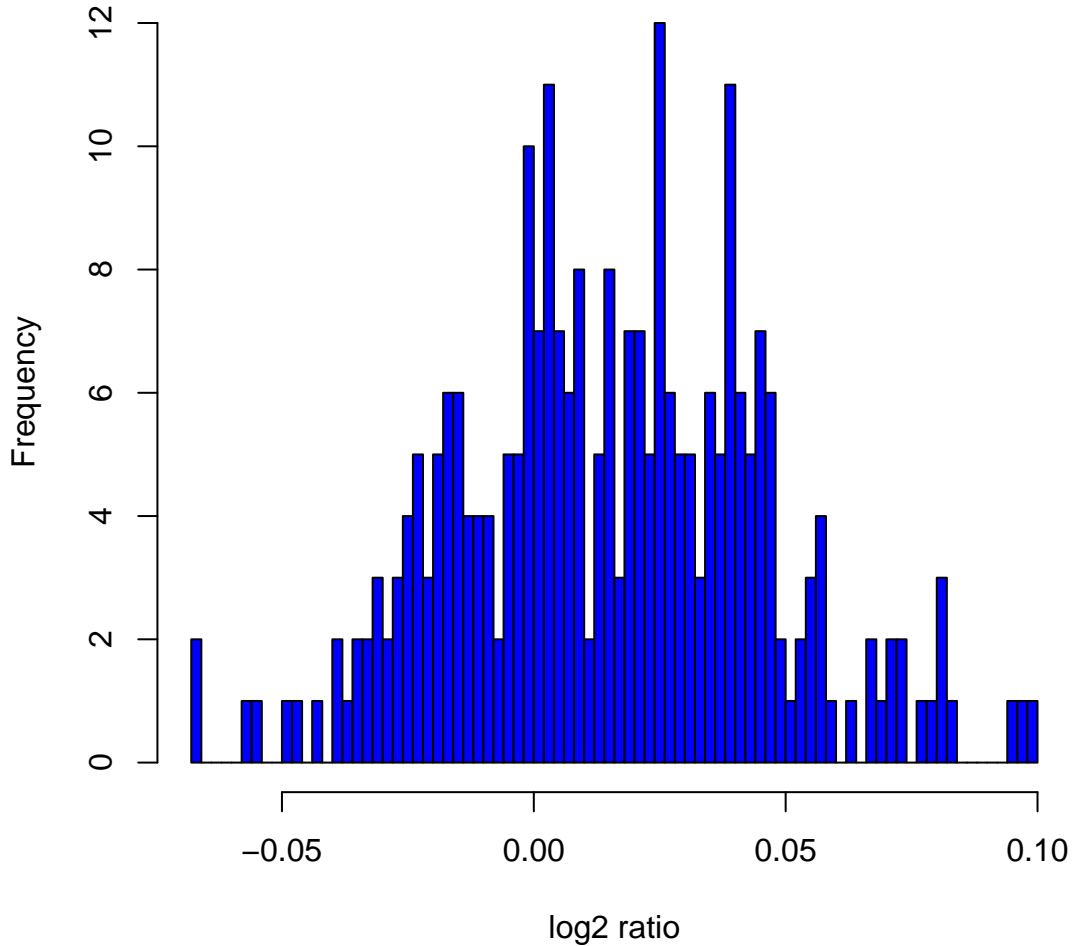
Histogram of log2ratios in 270 HapMap samples at clone Chr10tp-8G5
