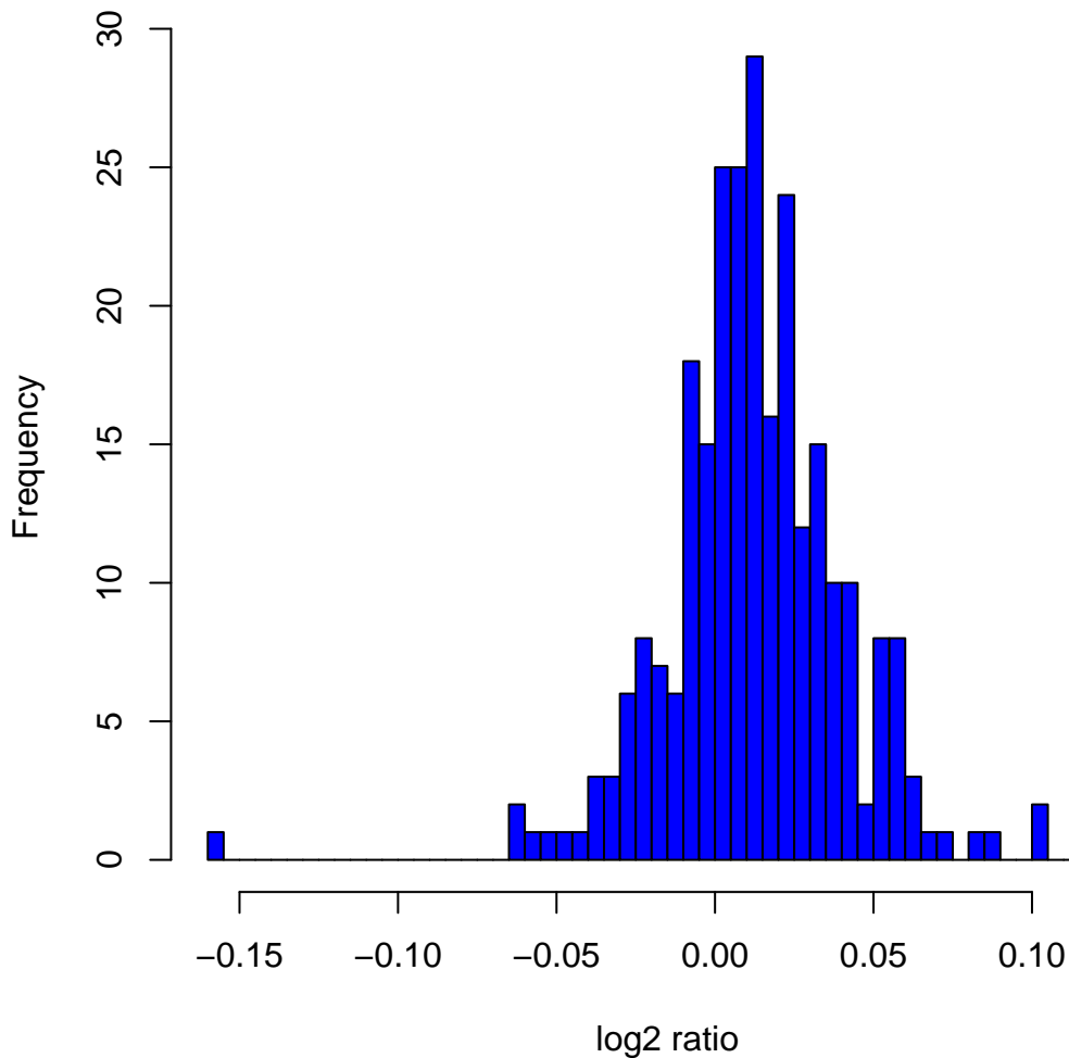
Histogram of log2ratios in 270 HapMap samples at clone Chr10tp-9A12
