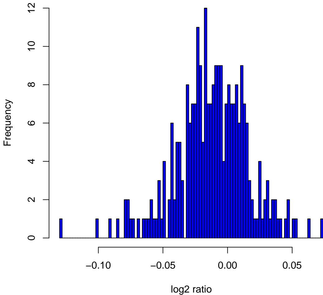
Histogram of log2ratios in 270 HapMap samples at clone Chr10tp-9D10
