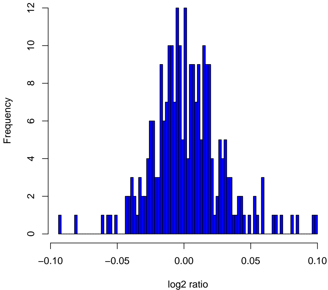
Histogram of log 2 ratios in 270 HapMap samples at clone Chr10tp-9G5
